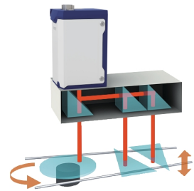
Multi spot measurement is available with splitting an optical axis 2 or 3.
